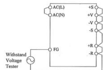
( C ) HWS100A,HWS150A
