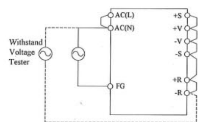
( C ) HWS100A,HWS150A
