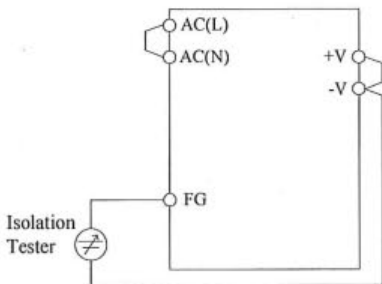
( A ) HWS15A,HWS30A
