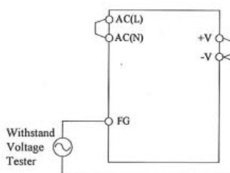
( A ) HWS15A,HWS30A
