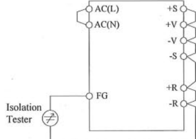
( C ) HWS100A,HWS150A
